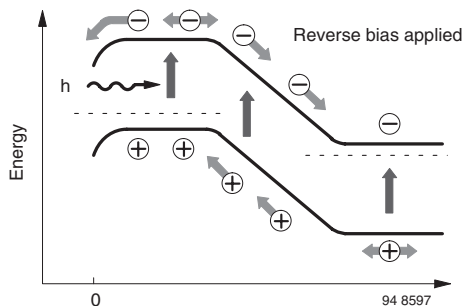
Fig. 9 - Generation-Recombination Effects in the Vicinity of a PN Junction Top: Short Circuit Mode, Bottom: Reverse Biased
