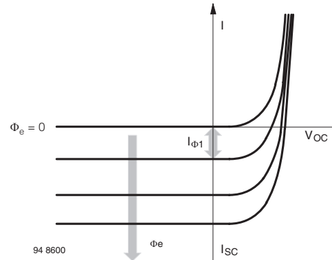
Fig. 12 - I-V-Charachteristics of an Si Photodiode under Illumination. Parameter: Incident Radiant Flux
