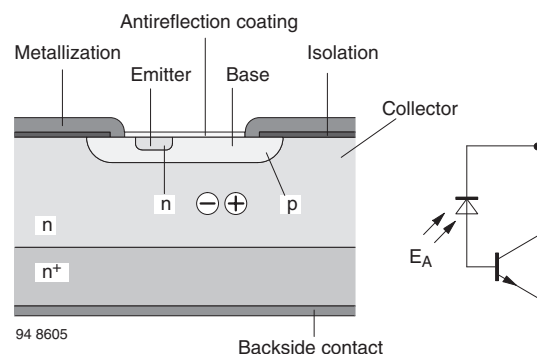
Fig. 15 - Phototransistor, Cross Section and Equivalent Circuit
